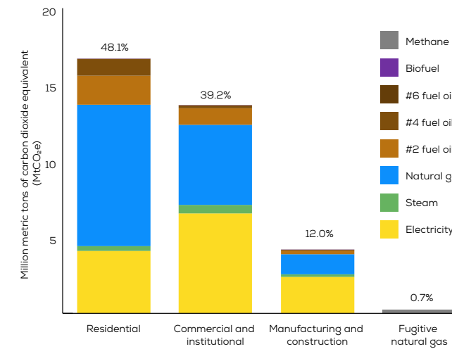
2016 CITYWIDE STATIONARY ENERGY GHG EMISSIONS BY SOURCE
